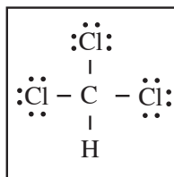
Chloroform, \text{CHCl}_3
